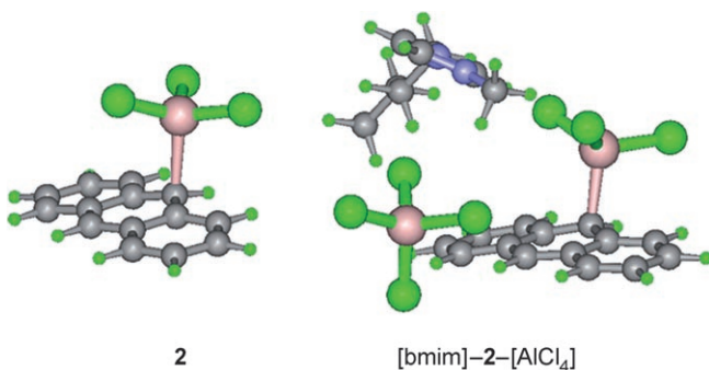
Figure 3. Computed structures of 2 and [bmim]–2–[AlCl 4 ].
