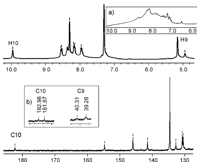
Figure 2. 1 H and 13 C NMR spectra (top and bottom) of the mixture of anthracene and 1 . a) 1 H NMR spectrum of a mixture of anthracene and AlCl 3 ; b) section of a proton coupled 13 C NMR spectra for the mixture of anthracene and 1 .
